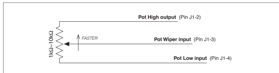
Fig. 7 Wiring for 3-wire potentiometer throttle (“Type 3”).
