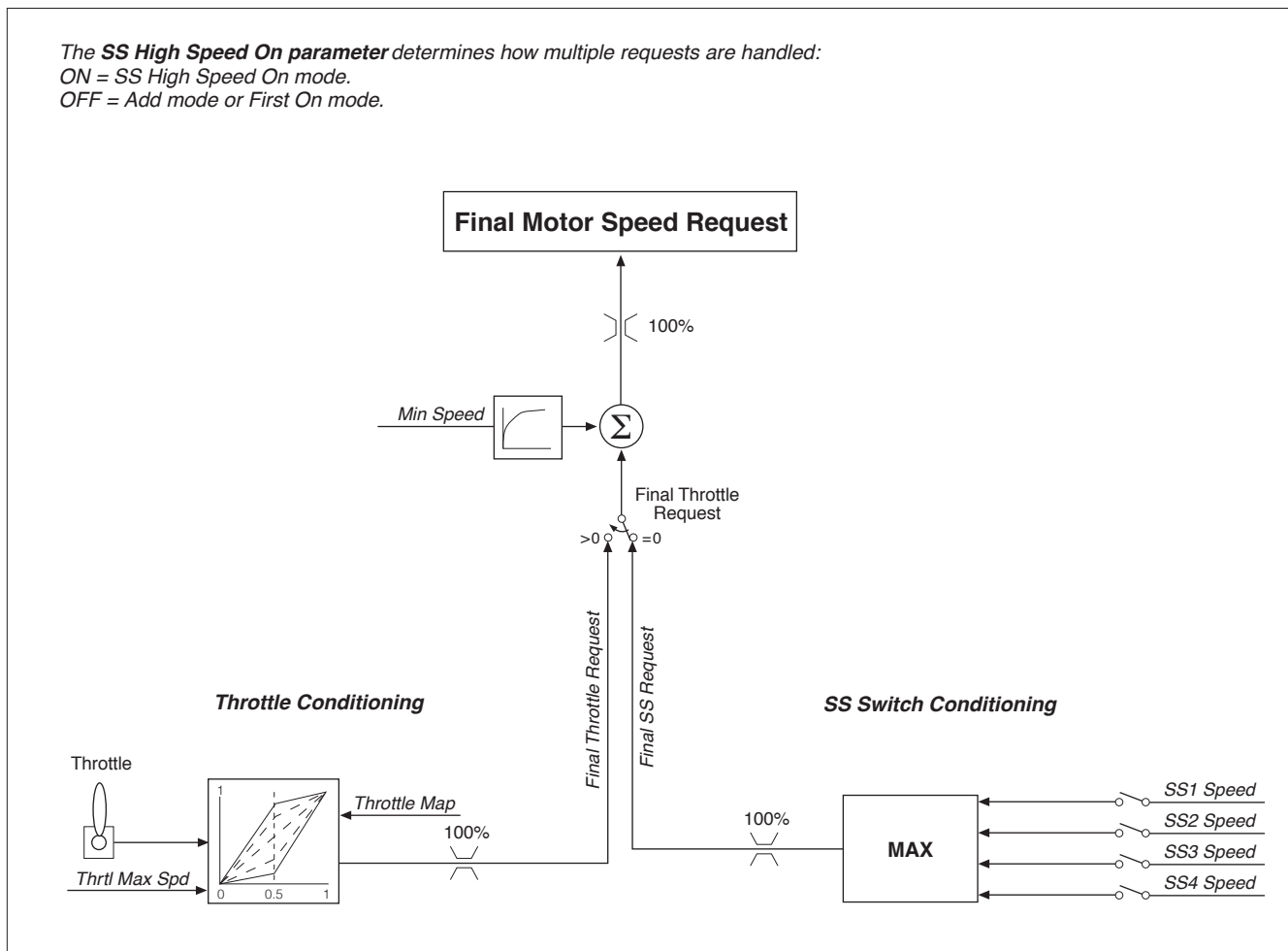
Fig. 14 SS High Speed On speed conditioning diagram.
