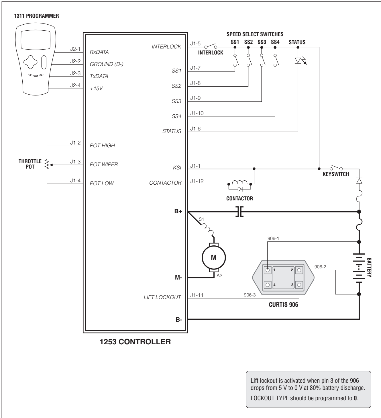
Fig. 3b Standard wiring configuration, Curtis 1253 controller with Curtis 906 providing lift lockout.
