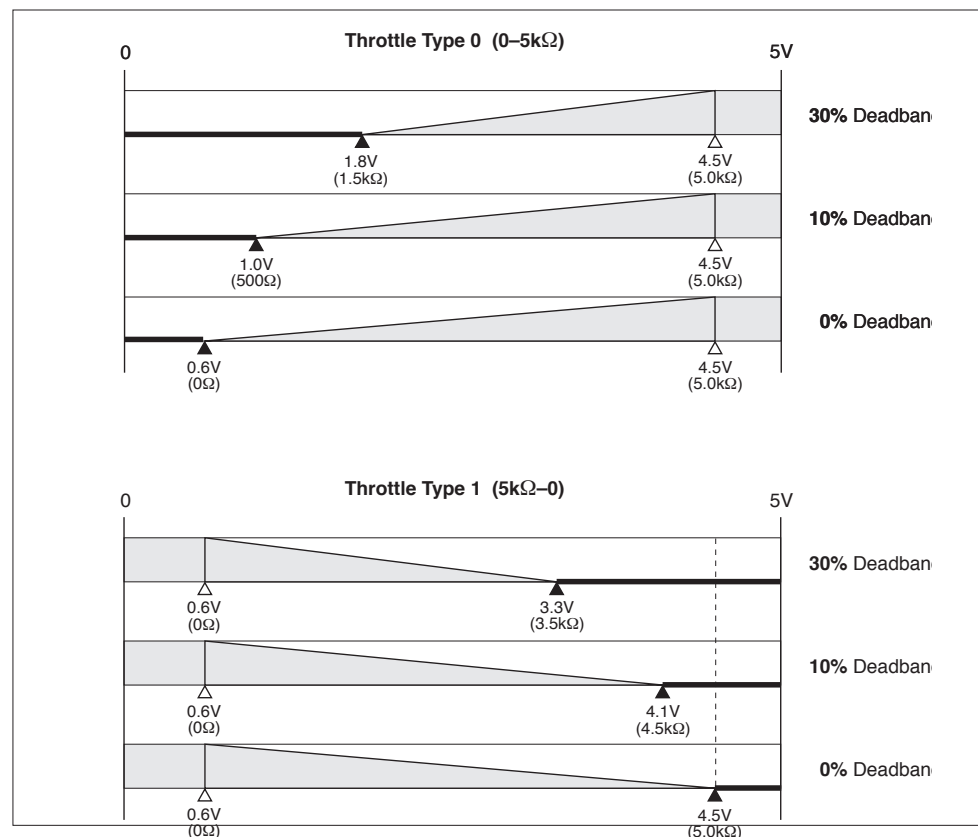
Fig. 8 Effect of adjusting the throttle deadband parameter (throttle types 0 and 1).
